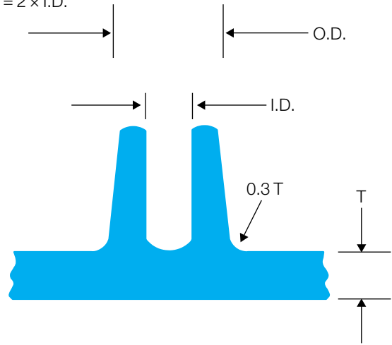
Figure 8.18 Boss design - general guidelines
