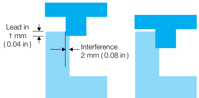
Figure 10.6 Shear joint
