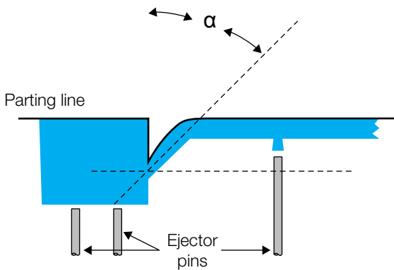
Figure 9.19 Tunnel gate
