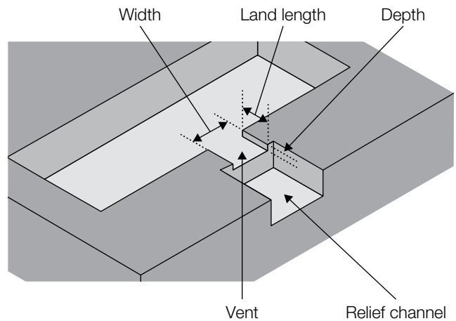
Figure 9.20 Vents
