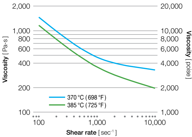
Figure 9.9 KetaSpire® KT-820 SL45
