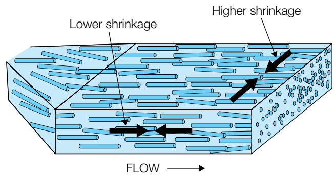
Figure 9.17 Shrinkage varies with flow direction
