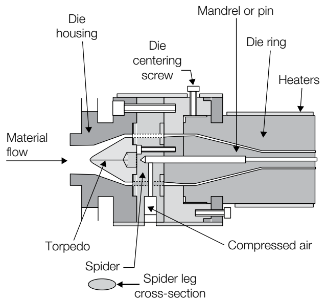
Figure 9.26 Tubing die
