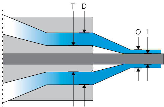
Figure 9.32 Sleeve die draw down ratio
