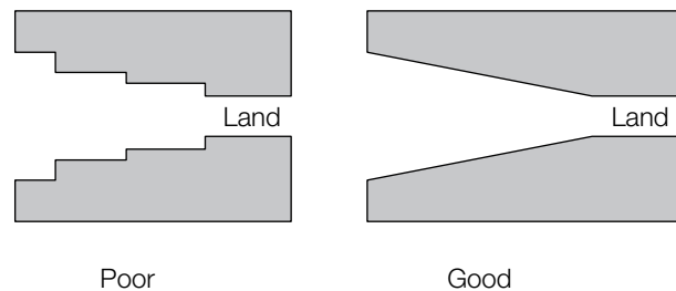
Figure 9.23 Adapter design
