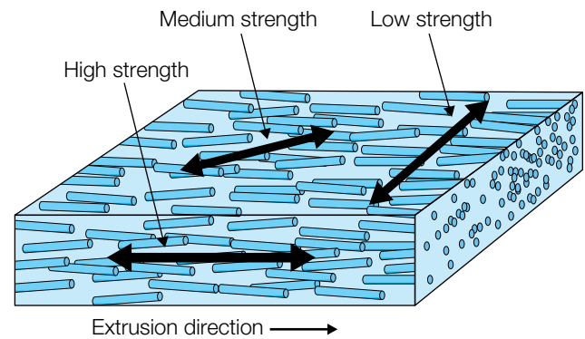
Figure 10.12 Fiber orientation affects strength
