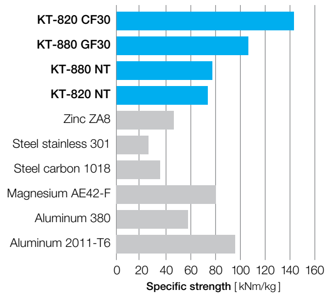
Figure 8.1 Specific strength
