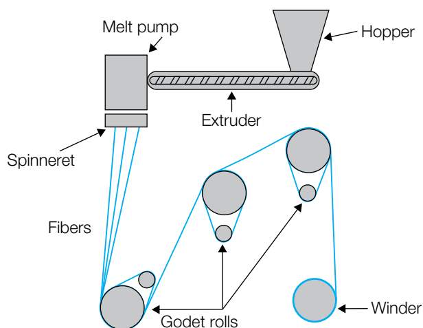
Figure 9.28 Fiber spinning process
