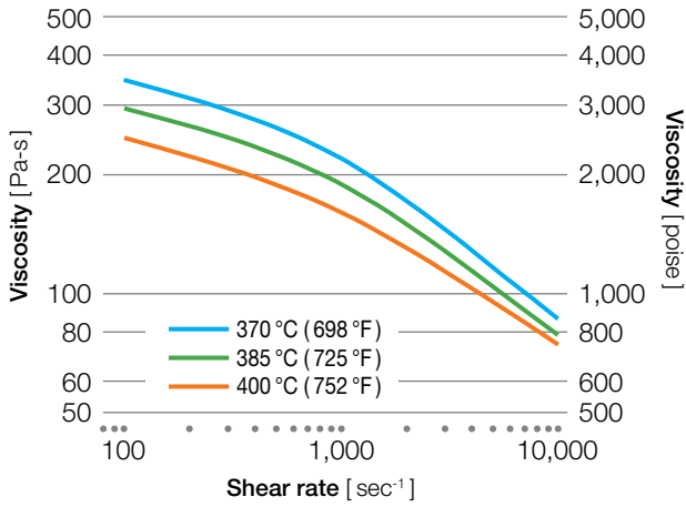
Figure 9.3 KetaSpire® KT-820 GF30
