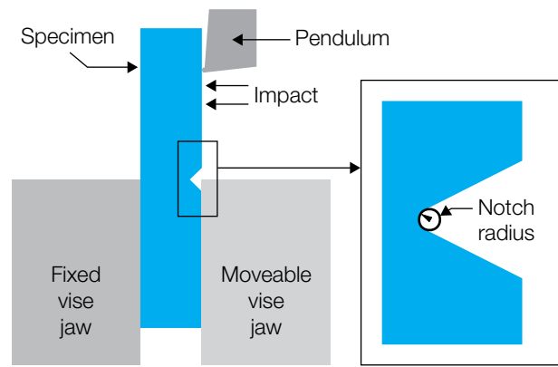
Figure 3.27 Notched Izod specimen
