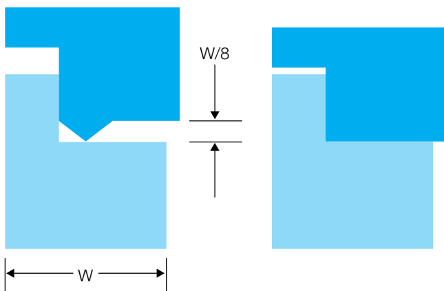
Figure 10.4 Step joint
